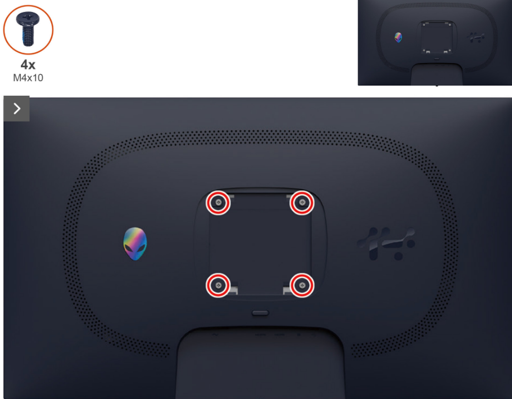
Figure 13. Removing the back cover
