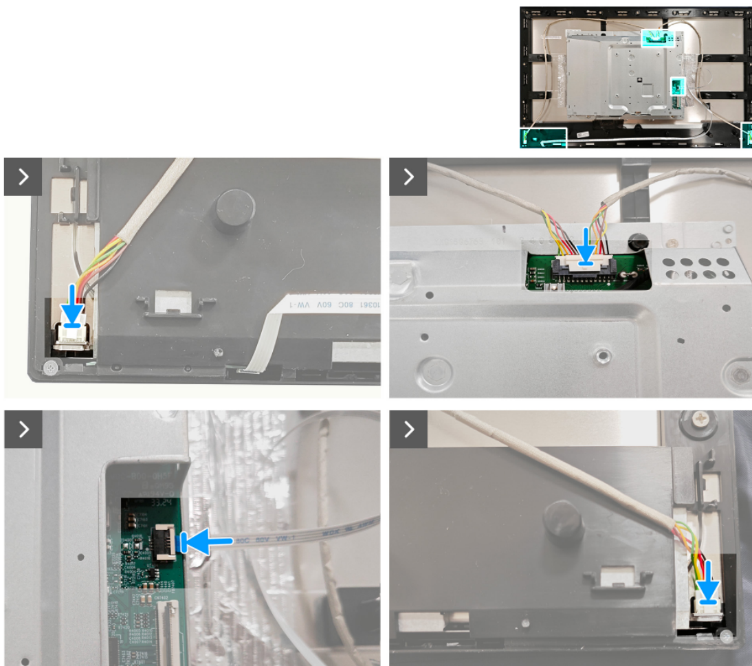
Figure 28. Installing the metal shield
