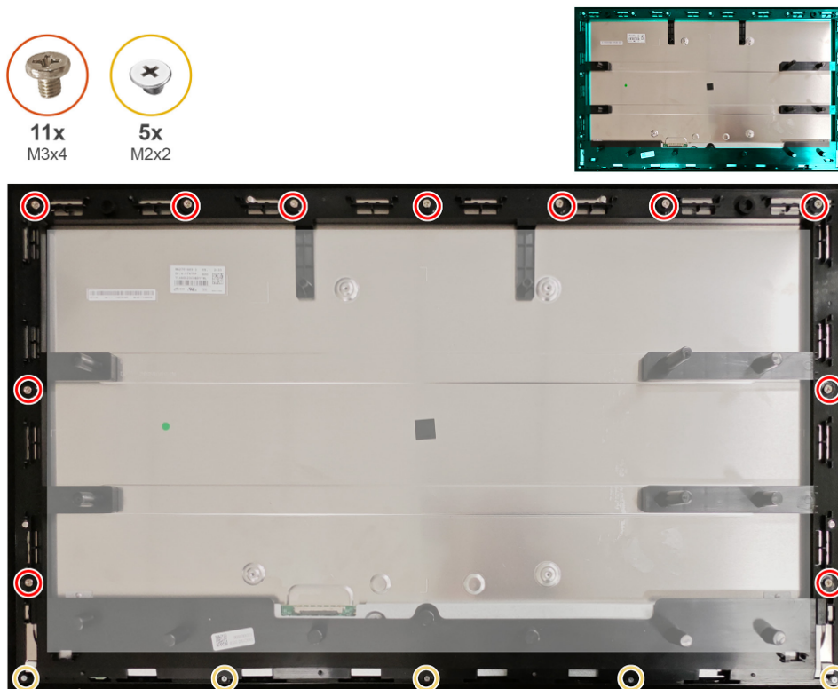
Figure 37. Installing the middle frame
